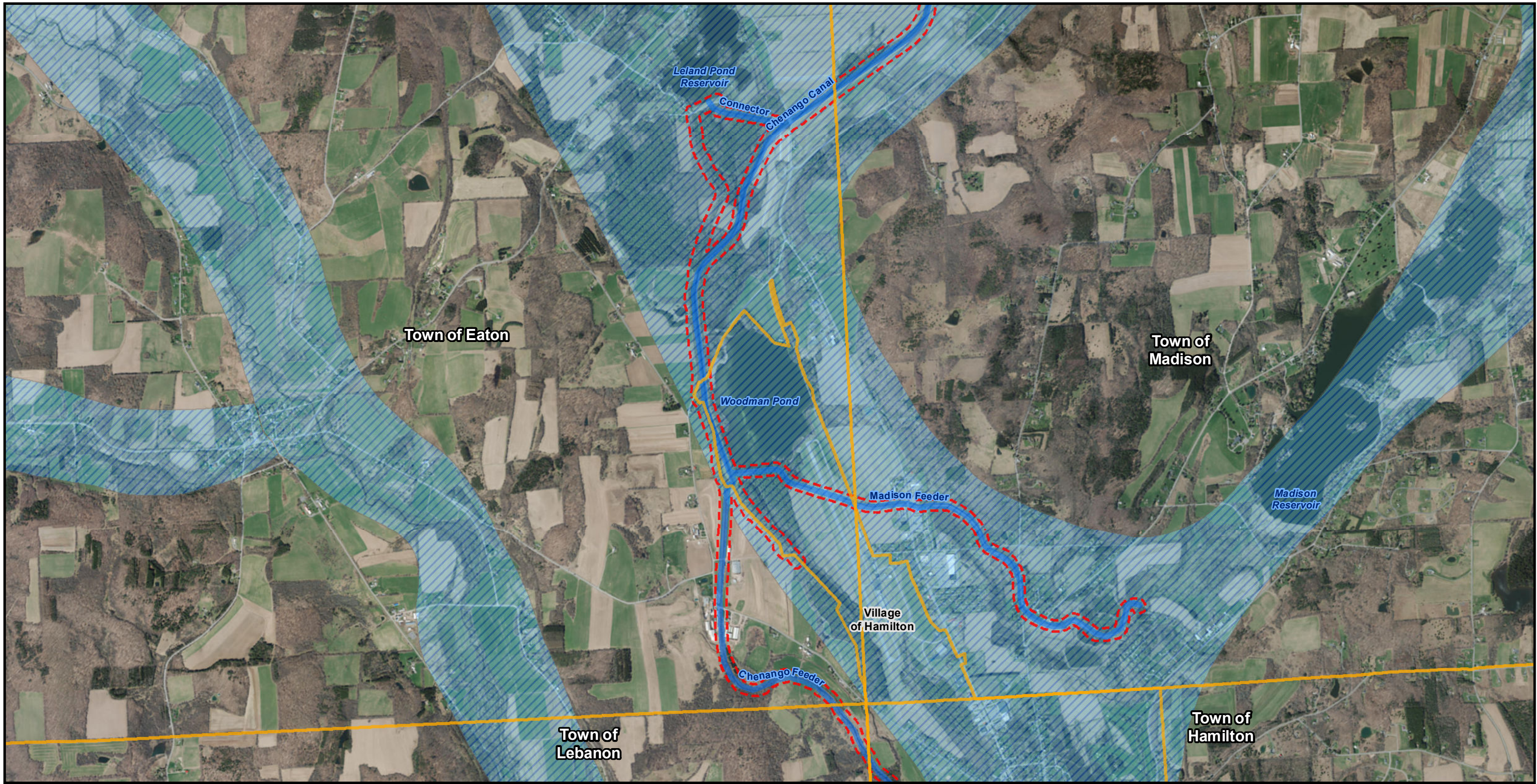
Figure 54F: Aquifers
